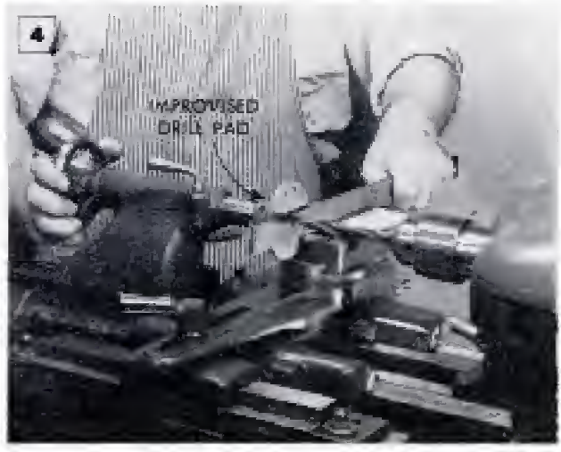
In live drilling, pictured in the photos above and below, the drill usually is held in a geared chuck and driven by the lathe headstock. Flat work is supported by a pad as in the lower views. Note wooden facing
